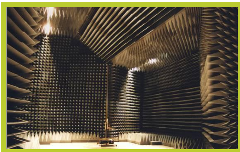
Hands-on session: EMC Measurement in Anechoic Chamber
